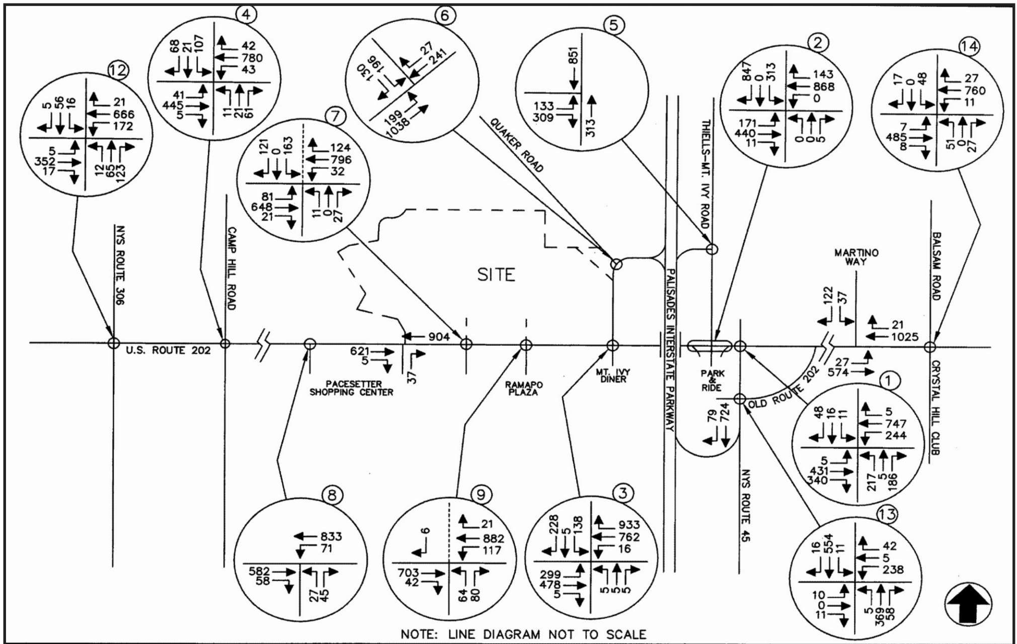
Figure 3.5-24: 2011 Build Traffic Volumes Weekday Peak AM Highway Hour (W/O Patrick Farm) Minisceongo Park Towns of Haverstraw & Ramapo, Rockland County, New York Source: John Collins Engineers, P.C. Date: October, 2008
